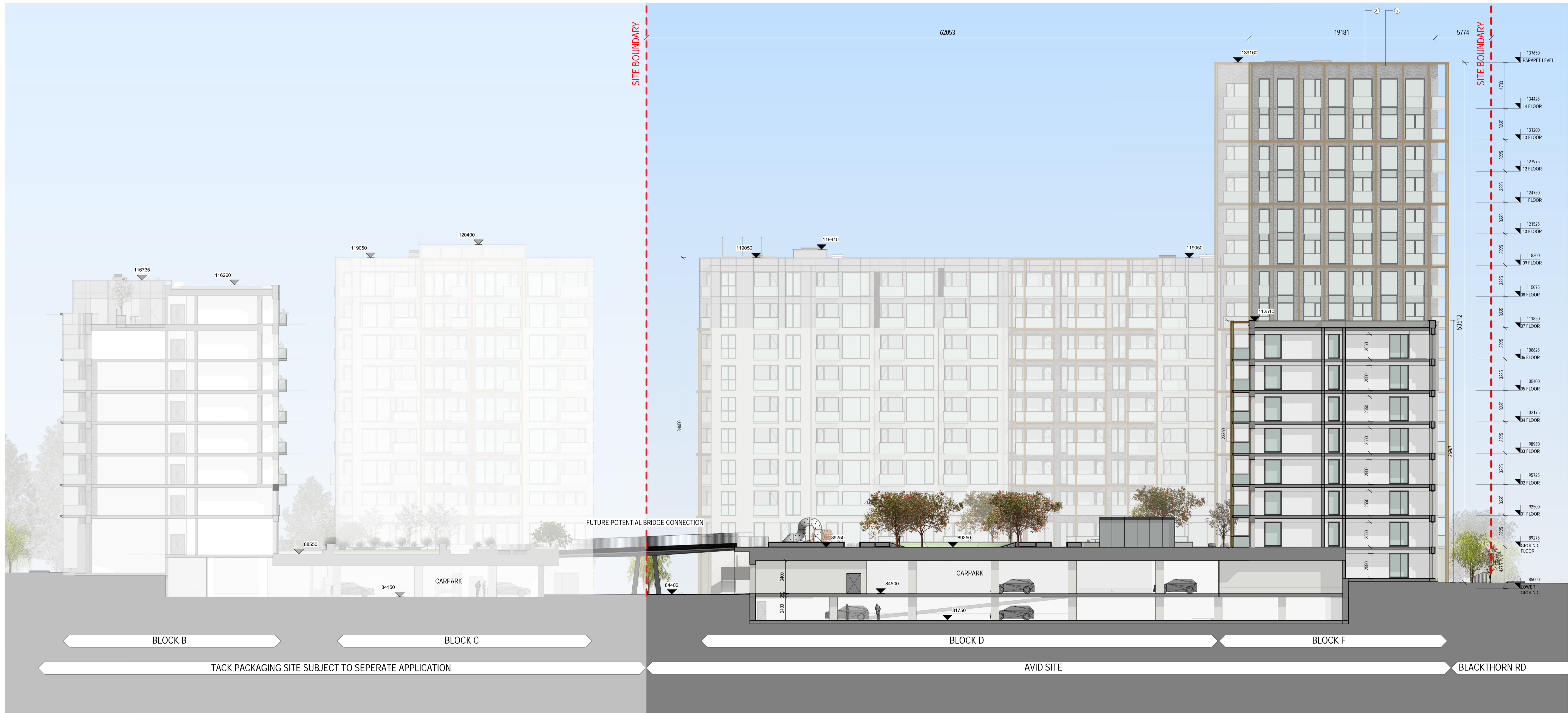
1 SECTION THROUGH PODIUM 01 - AVID SITE 1:200
